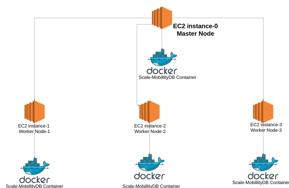
Scaling MobilityDB using Citus data cluster
